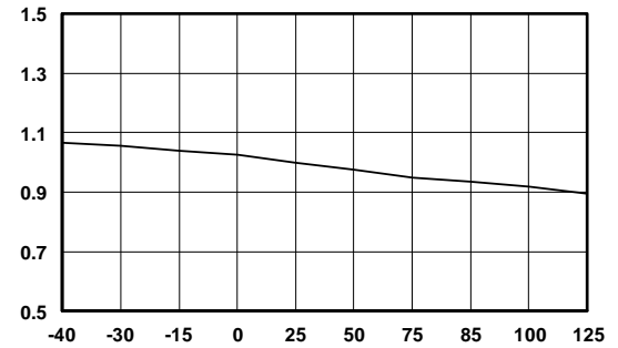
Figure 10. f_{MIN-CC} vs. Temperature
