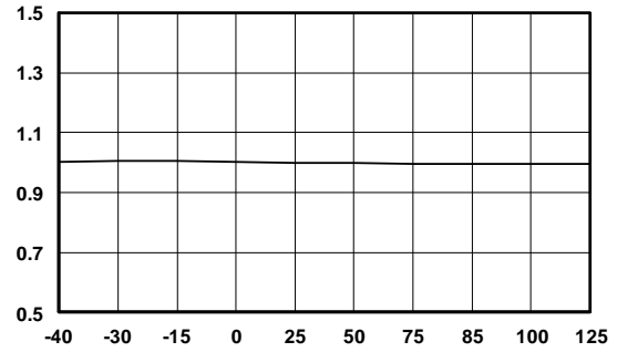
Figure 8. V_{OVp} vs. Temperature
