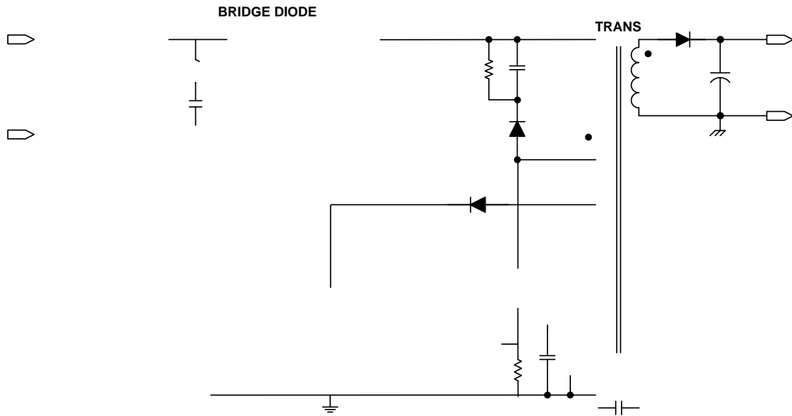
Figure 1. Typical Application
