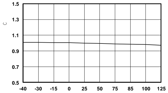
Figure 6. V_{DD-OFF} vs. Temperature
