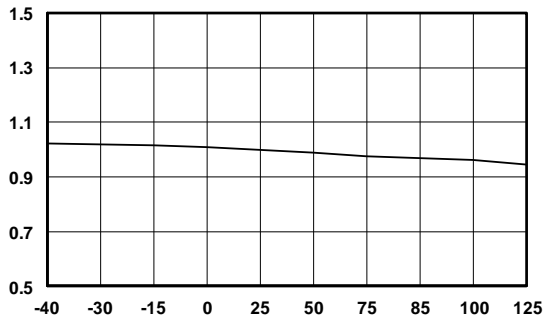
Figure 5. V_{DD-ON} vs. Temperature
