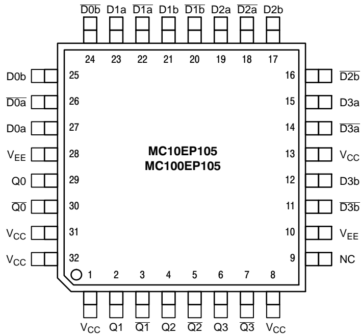
Fig re 1. 32-Lead LQFP Pino u(Top View)
